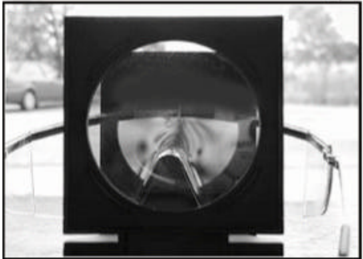
Viewing a pair of safety glasses through the Stress Indicator.
