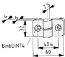
Part # 0002612 #8 Hinge PA, right
