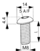
Part # 0019673 M8 x 20 Button Head Screw
