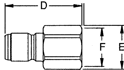
F = Across Flats E = Across Corners
